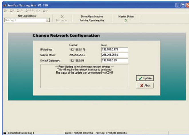
Fig 10-6: Network Settings
