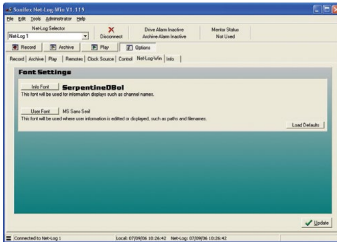
Fig 9-8: Net-Log-Win Options
