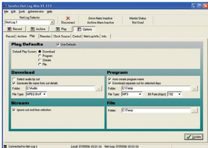
Fig 9-3: Play Options
