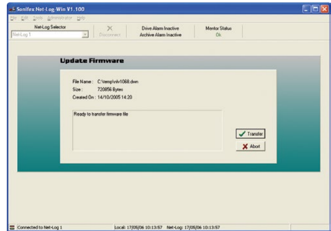
Fig 10-7: Upgrading Firmware
