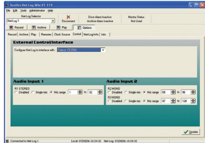
Fig 9-7: Televic CE2500 Control Options
