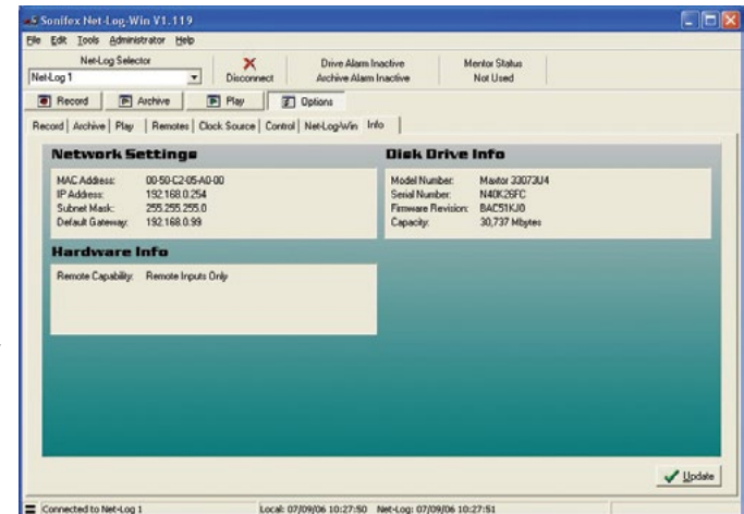
Fig 9-9: Info Options
