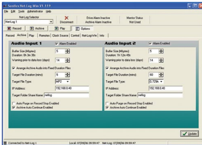
Fig 9-2: Archive Options
